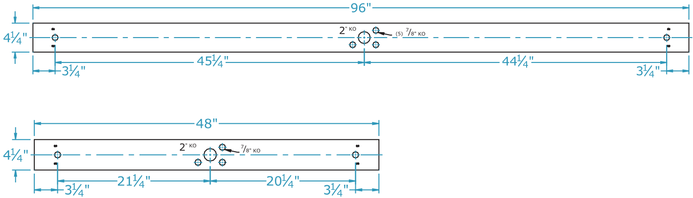
Back View
