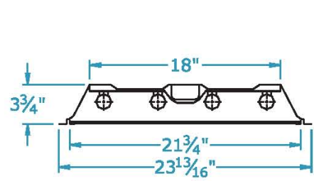
2x2 FOUR LAMP UNIT
