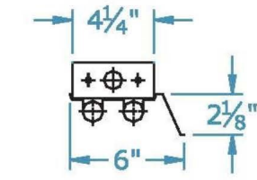
Asymmetrical Reflector
