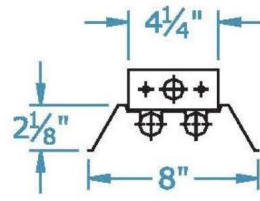
Symmetrical Reflector
