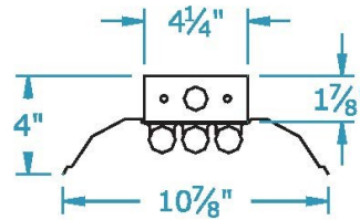
End View
