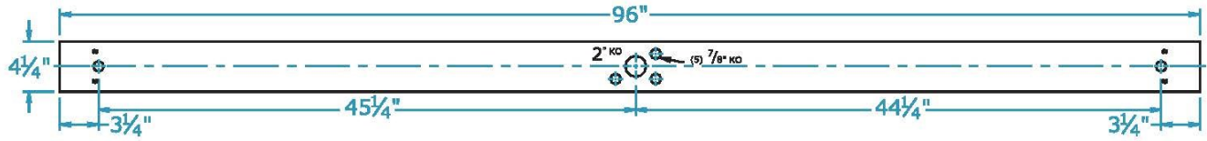
Back View
